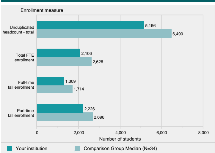
Figure 2. Unduplicated 12-month headcount (2009-10), total FTE enrollment (2009-10), and full- and part-time enrollment (Fall 2010) (ChartID: 2)
